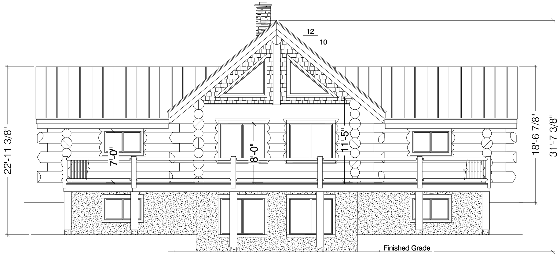
Front Elevation
