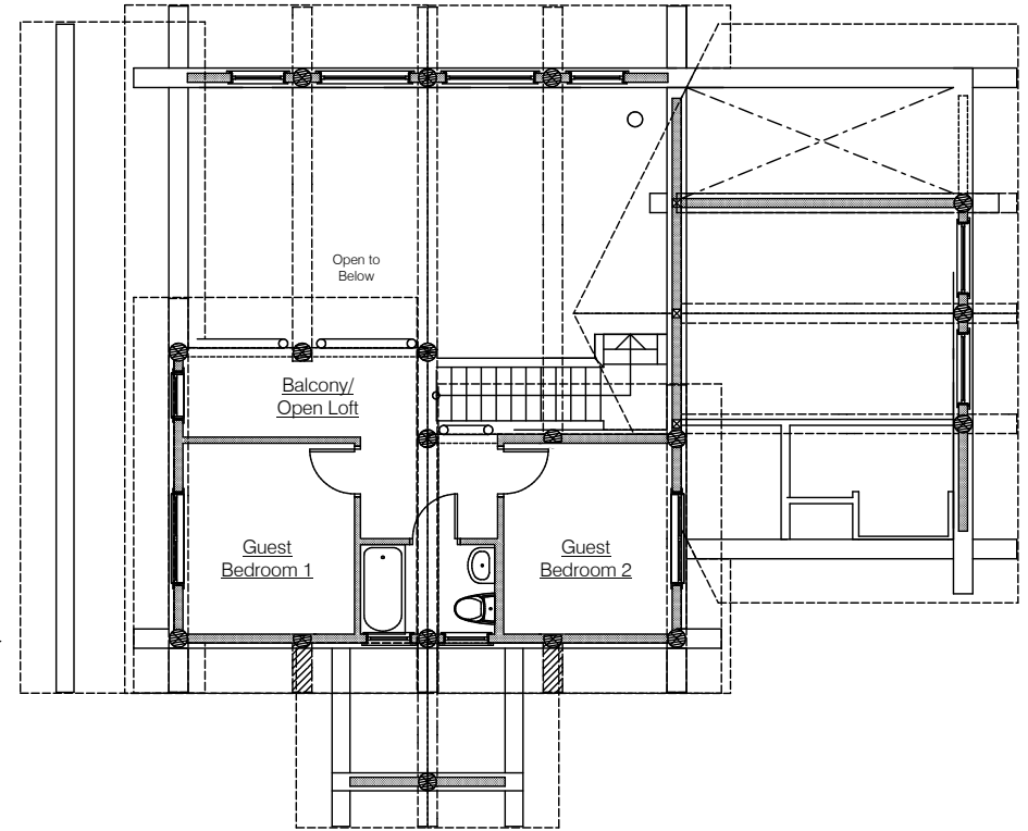
Loft Floor Plan 398 Sq. Ft. (over 6' headroom)
