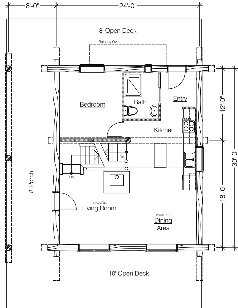
Main Floor Plan House - 756 Sq. Ft.
