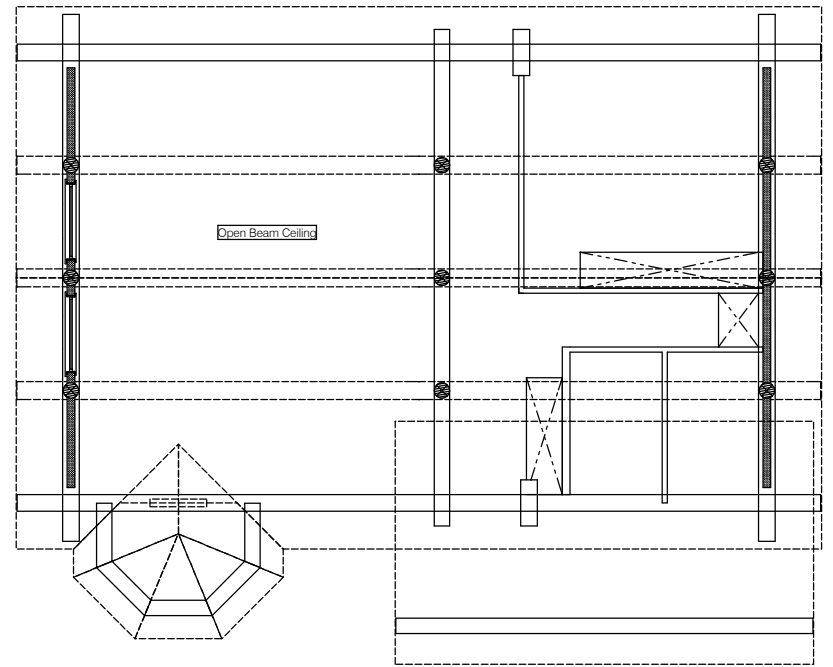
Roof Plan
