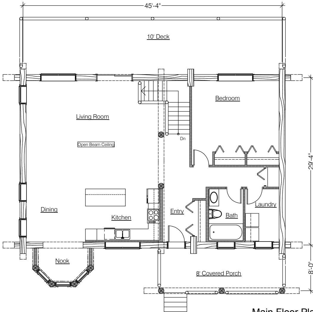
Main Floor Plan House - 1440 Sq. Ft.
