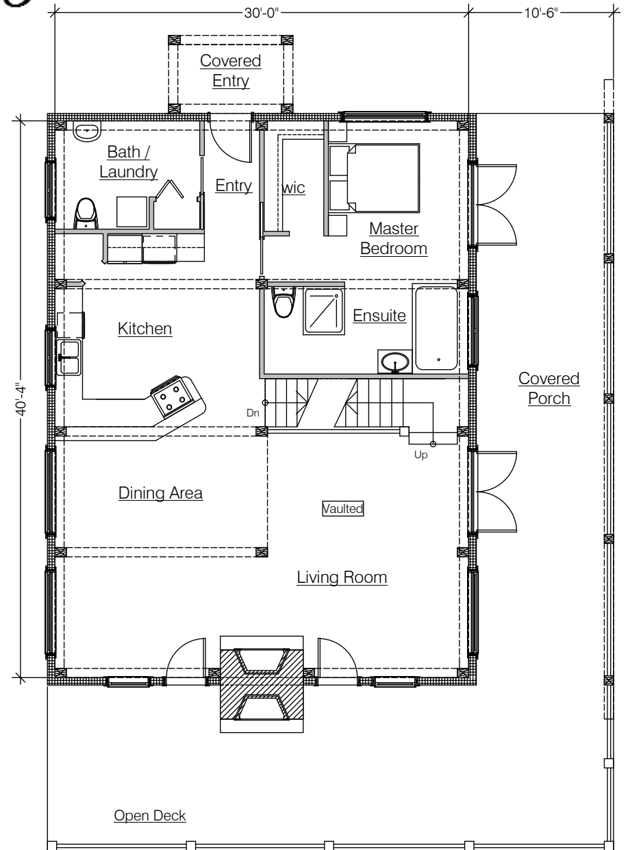
Main Floor 1282 Sq. Ft.
