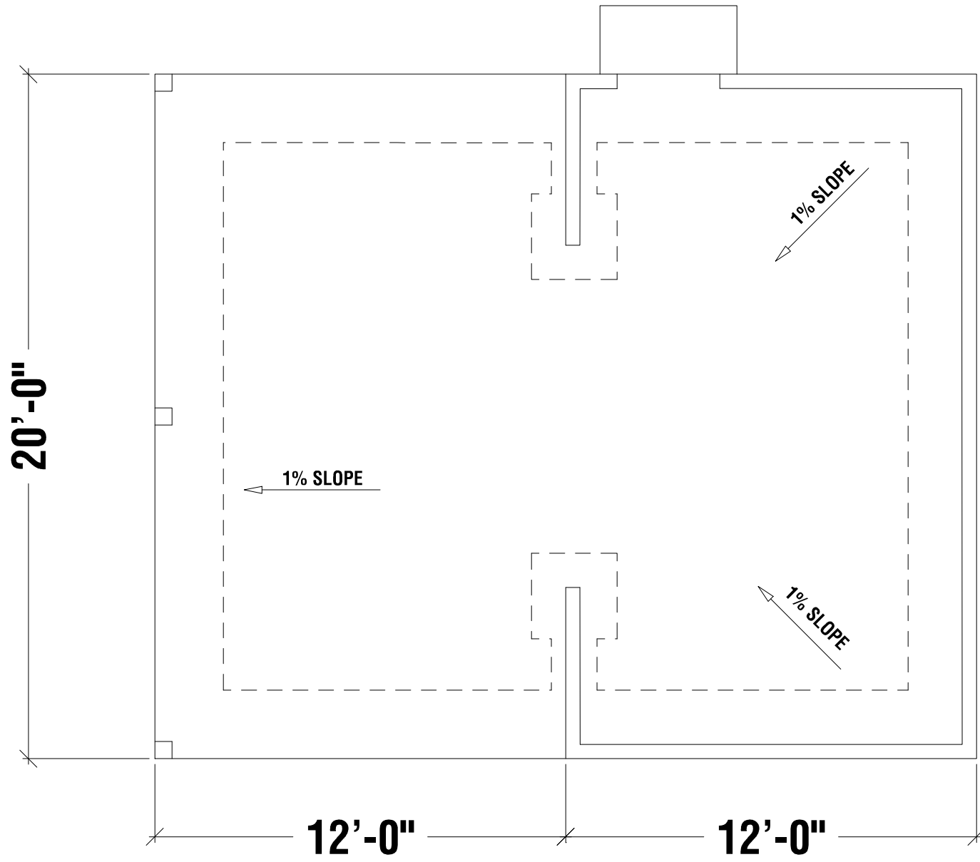
Foundation Plan
