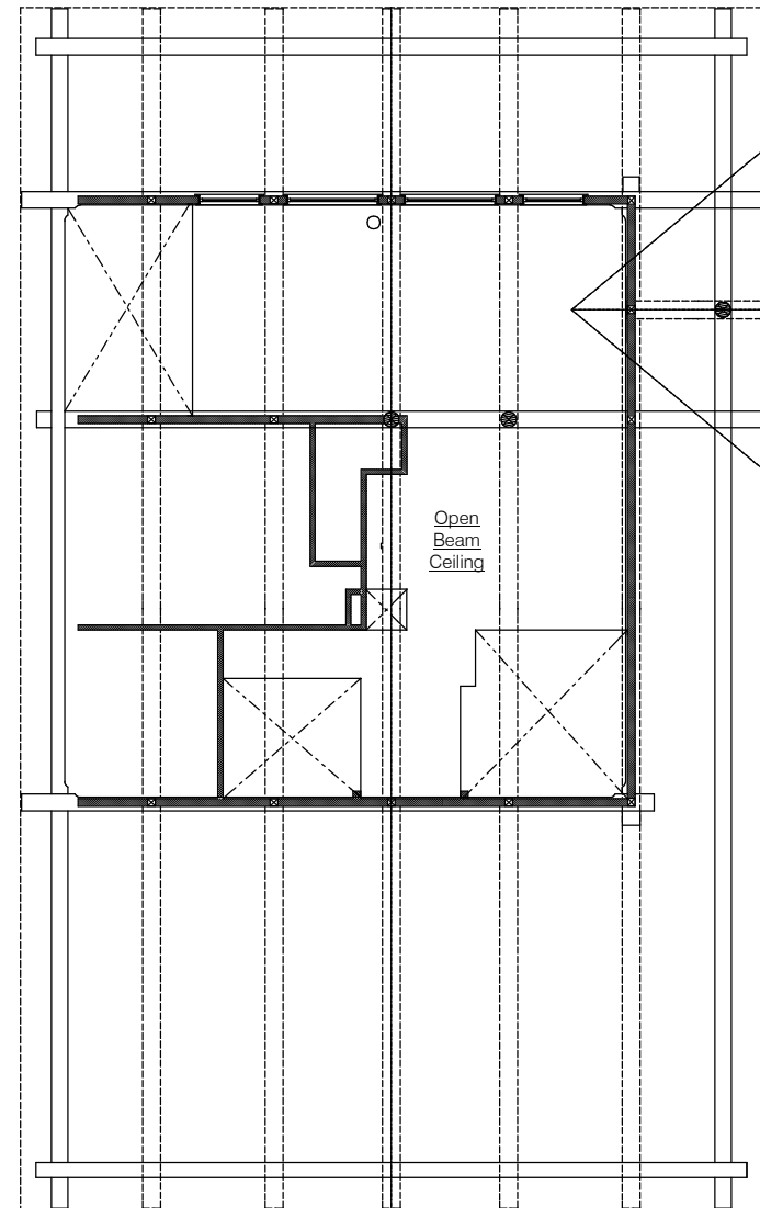
Roof Plan
