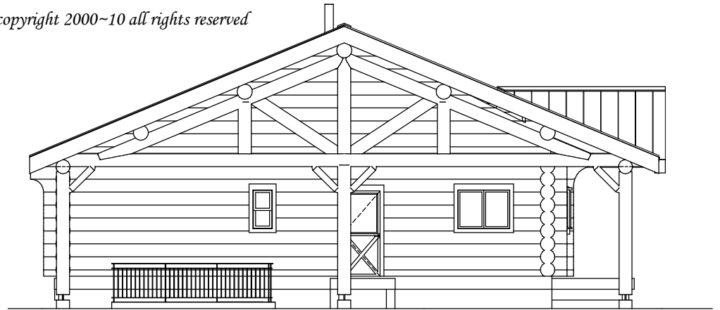
Front Elevation
