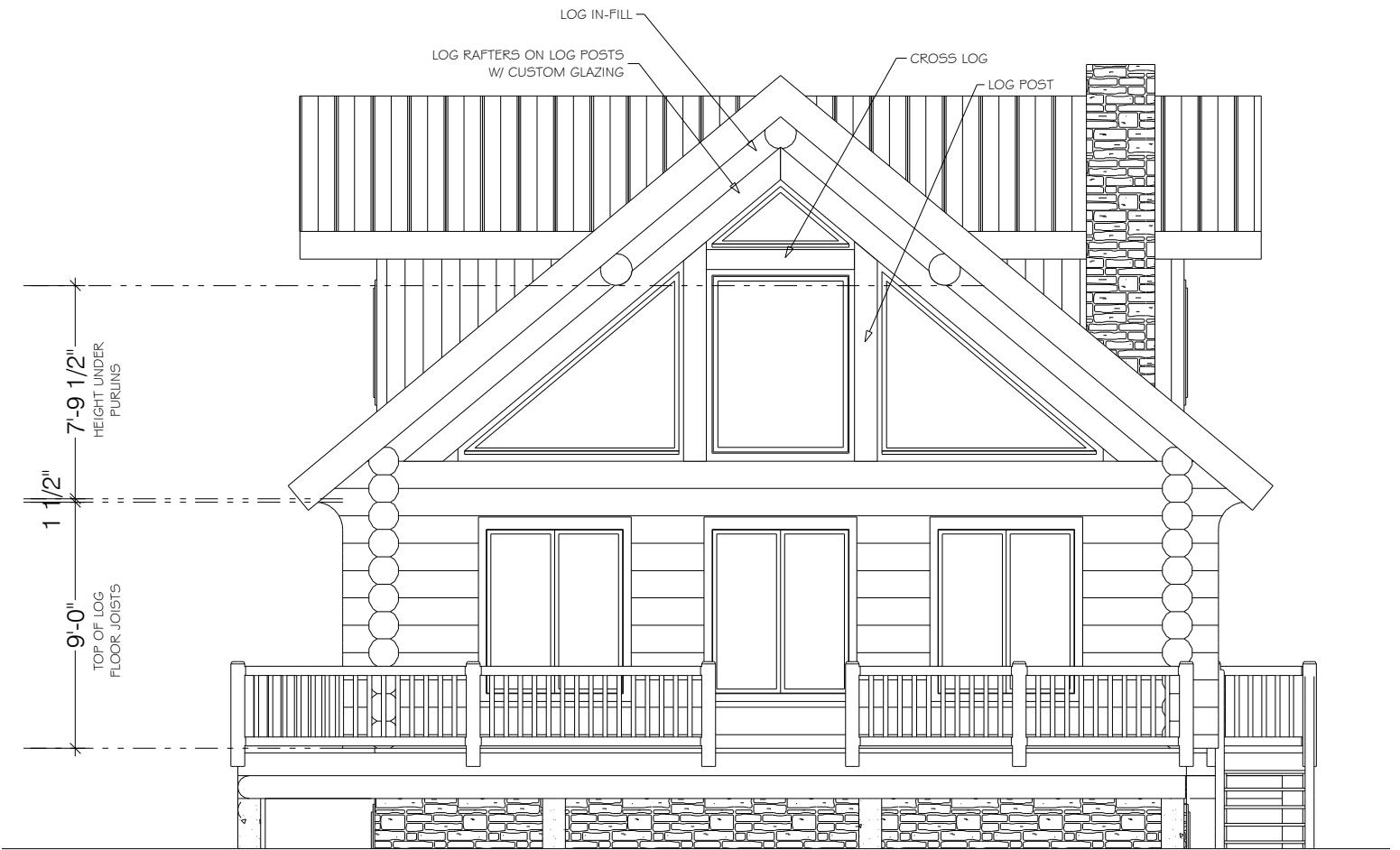
Front Elevation
