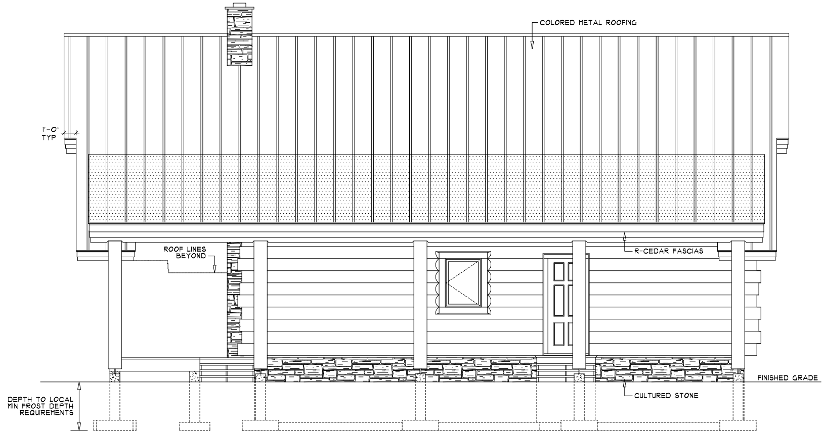
Left Elevation
