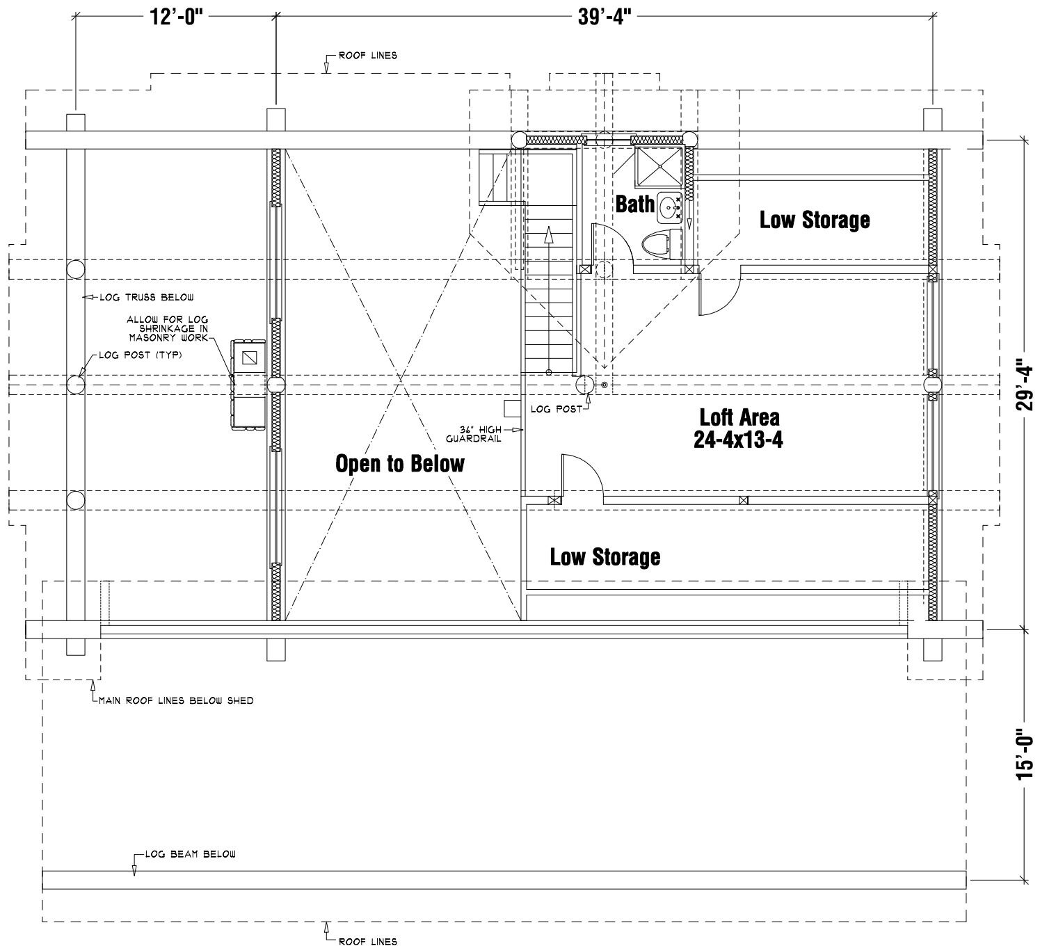
Loft Floor Plan 610 Sq.Ft.
