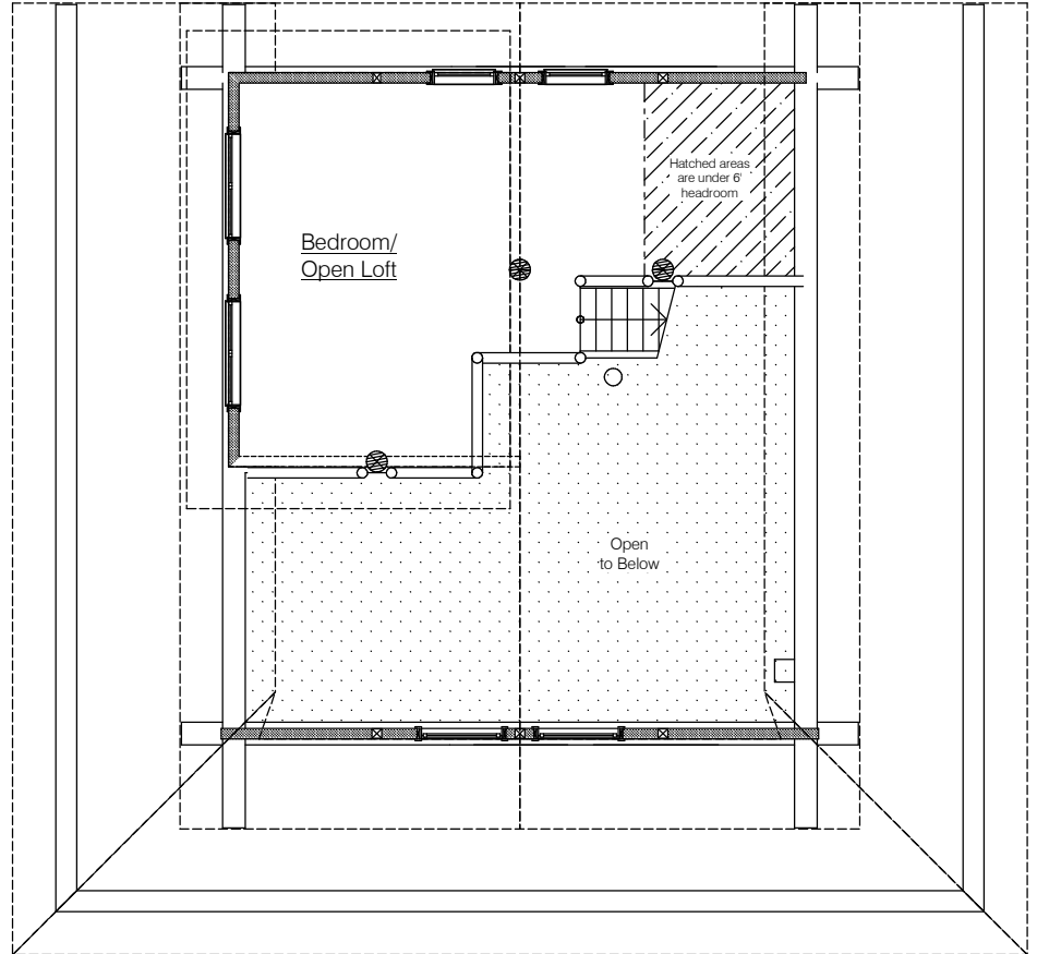
Loft Floor Plan 322 Sq. Ft. (over 6' headroom)
